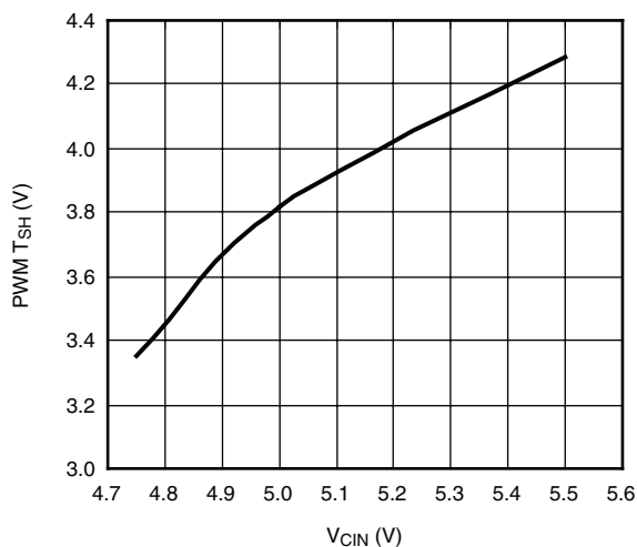
PWM Rising Threshold vs. V CIN
