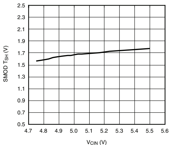
SMOD Rising Threshold vs. V CIN
