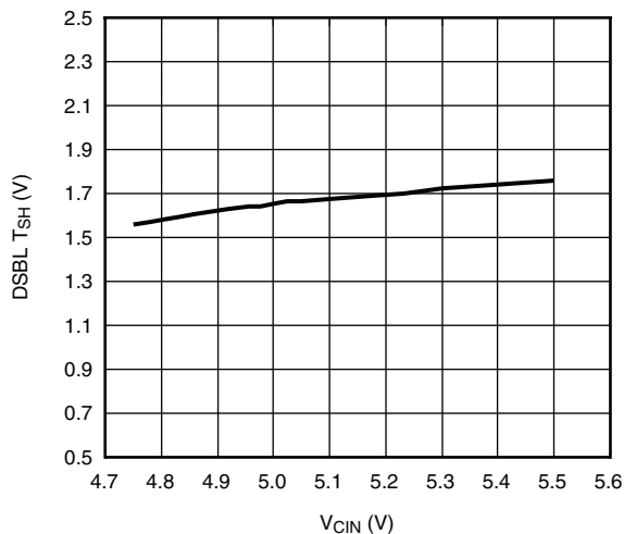
DSBL Rising Threshold vs. V CIN
