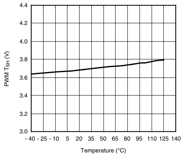
PWM Rising Tristate Threshold (V) vs. Temperature (°C) V_{CIN} = V_{DRV} = 5 V
