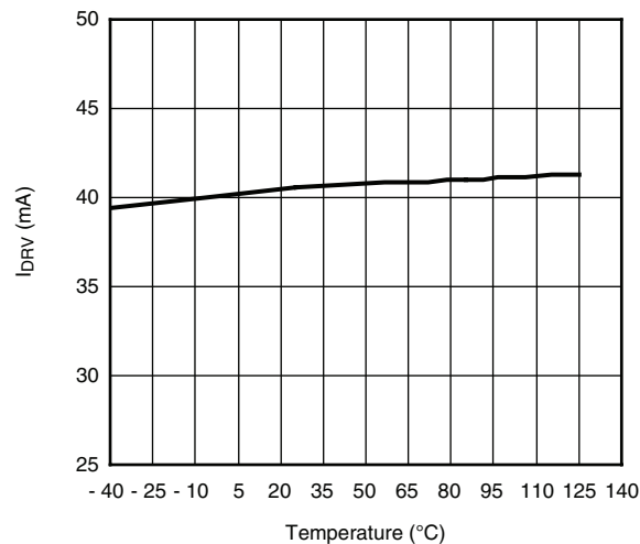
IDRV (mA) vs. Temperature at Frequency = 1 MHz D = 10 \%, V_{CIN} = V_{DRV} = 5 V
