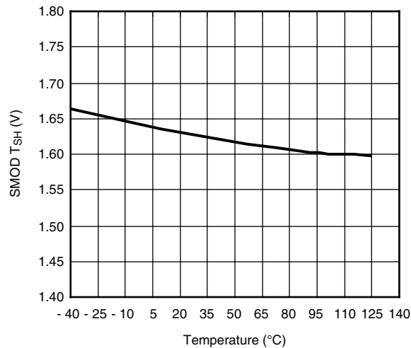
SMOD Rising Threshold (V) vs. Temperature (°C) V_{CIN} = V_{DRV} = 5 V
