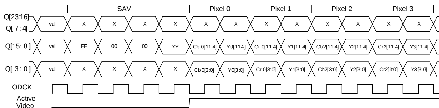
Figure 25. YCbCr Mux 4:2:2 Embedded Sync Encoding Timing Diagram
