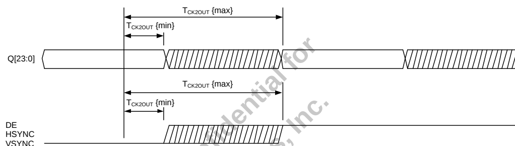
Figure 11. Receiver Clock-to-Output Delay and Duty Cycle Limits
