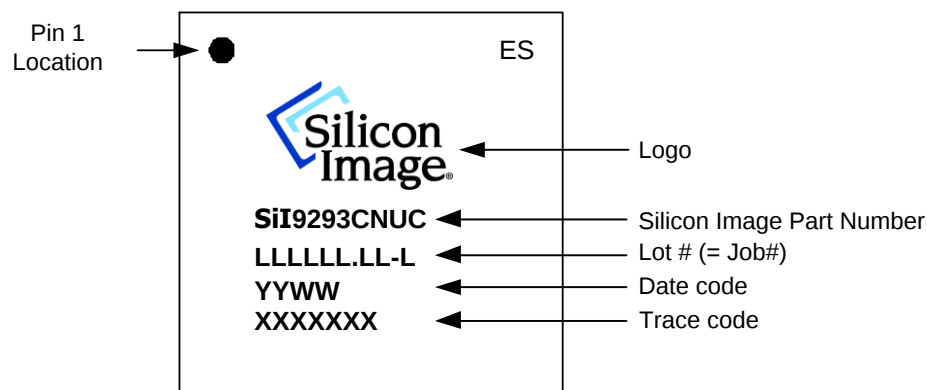
Figure 32. Marking Diagram
