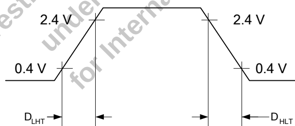
Figure 10. Video Digital Output Transition Times
