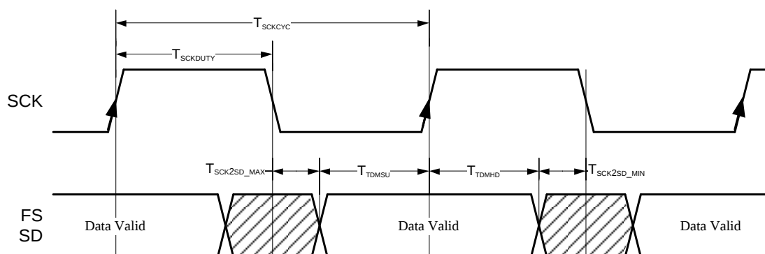
Figure 13. TDM Output Timings
