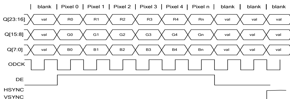
Figure 21. 4:4:4 Timing Diagram
