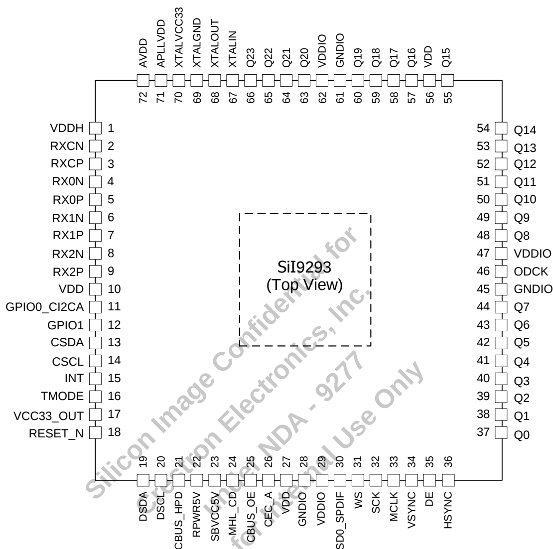
Figure 2. Pin Mapping
