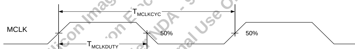
Figure 15. MCLK Timings
