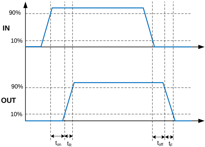
Figure 3. Switching Timing Waveform
