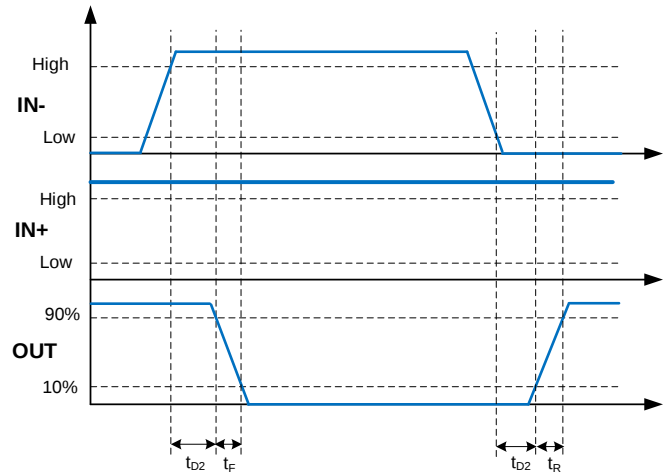
Figure 3. Inverting Configuration
