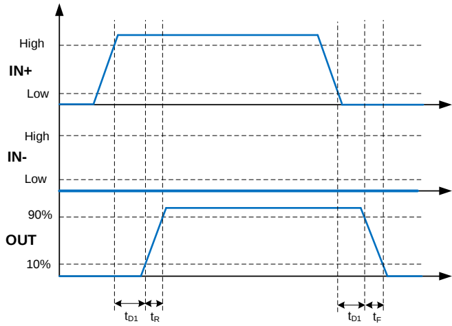
Figure 2. Noninverting Configuration
