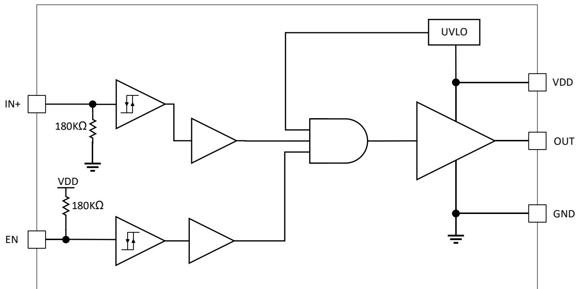
Figure 1. Function Block
