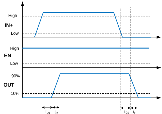
Figure 3. Noninverting Configuration
