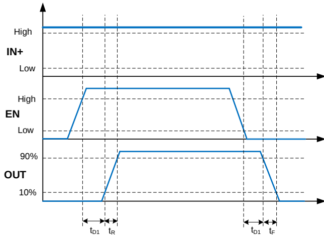
Figure 2. Enable and Disable Function Using EN Pin
