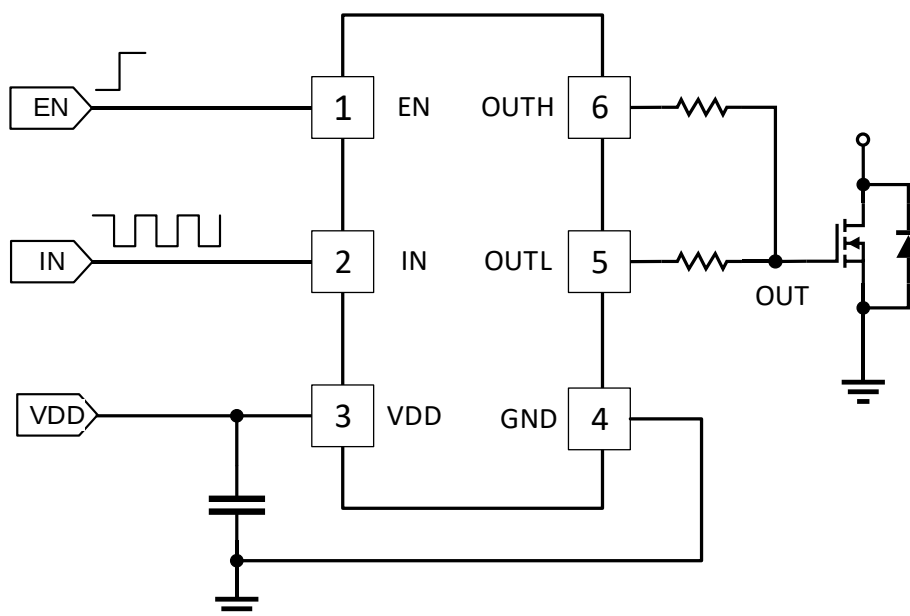
Figure 1. SiLM27531H-AQ Typical Application Circuit
