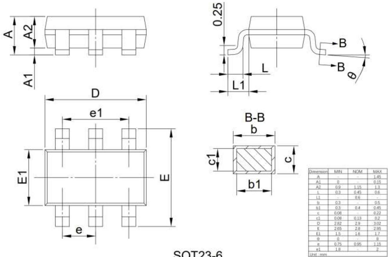
SOT23-6 Figure 5. SOT23-6 Outline Dimensions
