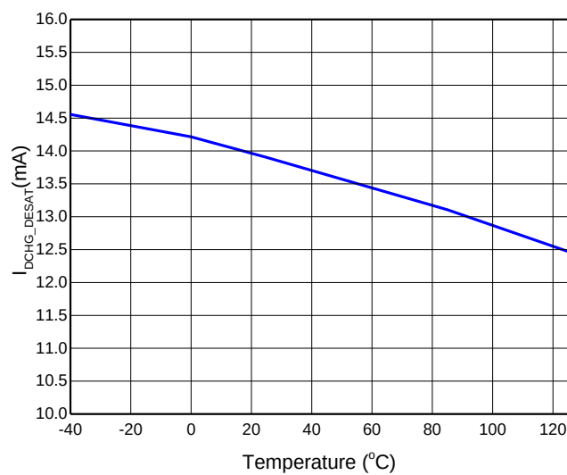
Figure 18. I_{DCHG\_DESAT} vs Temperature
