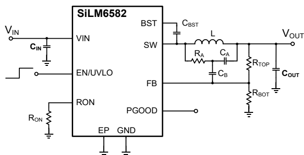
Figure 1. SiLM6582 Application Circuit
