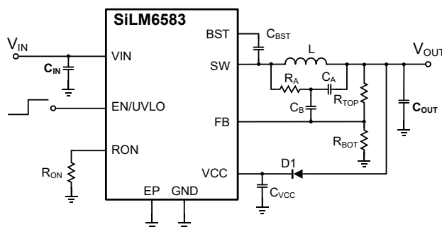
Figure 2 SiLM6583 Application Circuit
