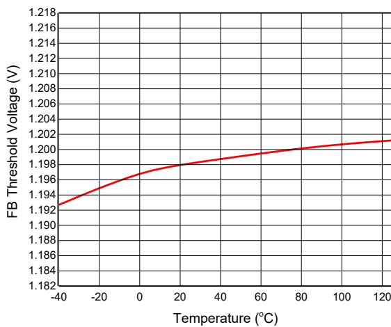
Figure 10. FB Threshold Voltage vs. Temperature
