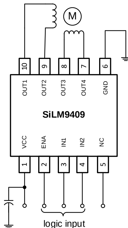
Figure 1. Typical Application Circuit
