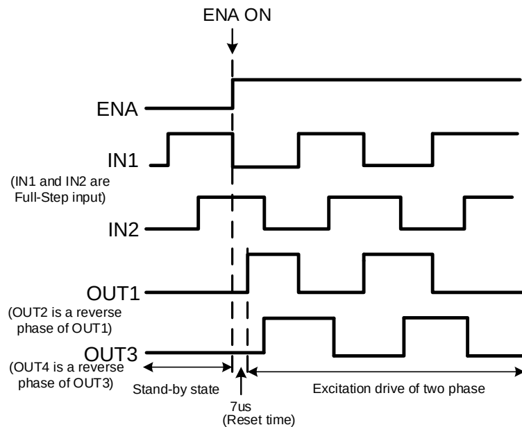
Figure 4. Control Timing
