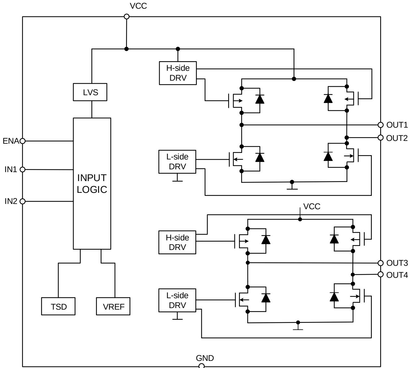
Figure 2. Block Diagram
