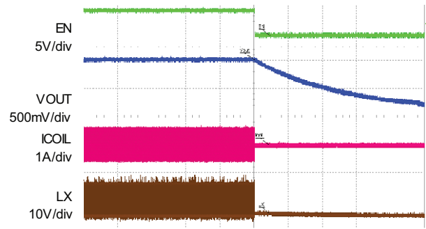
Fig. 14 - Shut-Down, I_{OUT} = 0\text{ A} , Time = 200 ms/div
