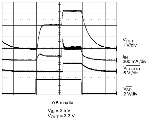
Figure 5. Turn On/Off Response ( V_{IN} = 2.5 V)
