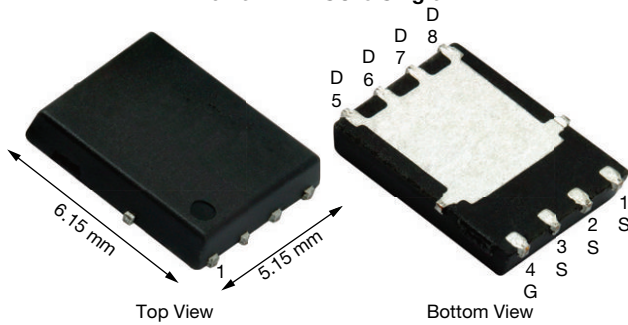
PowerPAK® SO-8 Single
