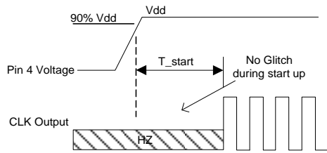
Figure 4. Startup Timing [11]
