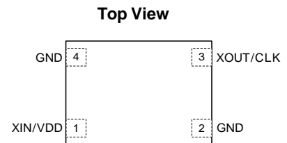
Figure 1. Pin Assignments
