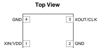
Figure 1. Pin Assignments
