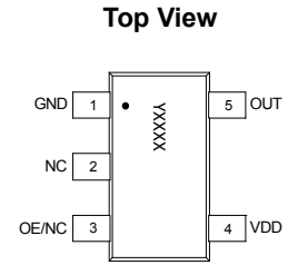
Figure 1. Pin Assignments
