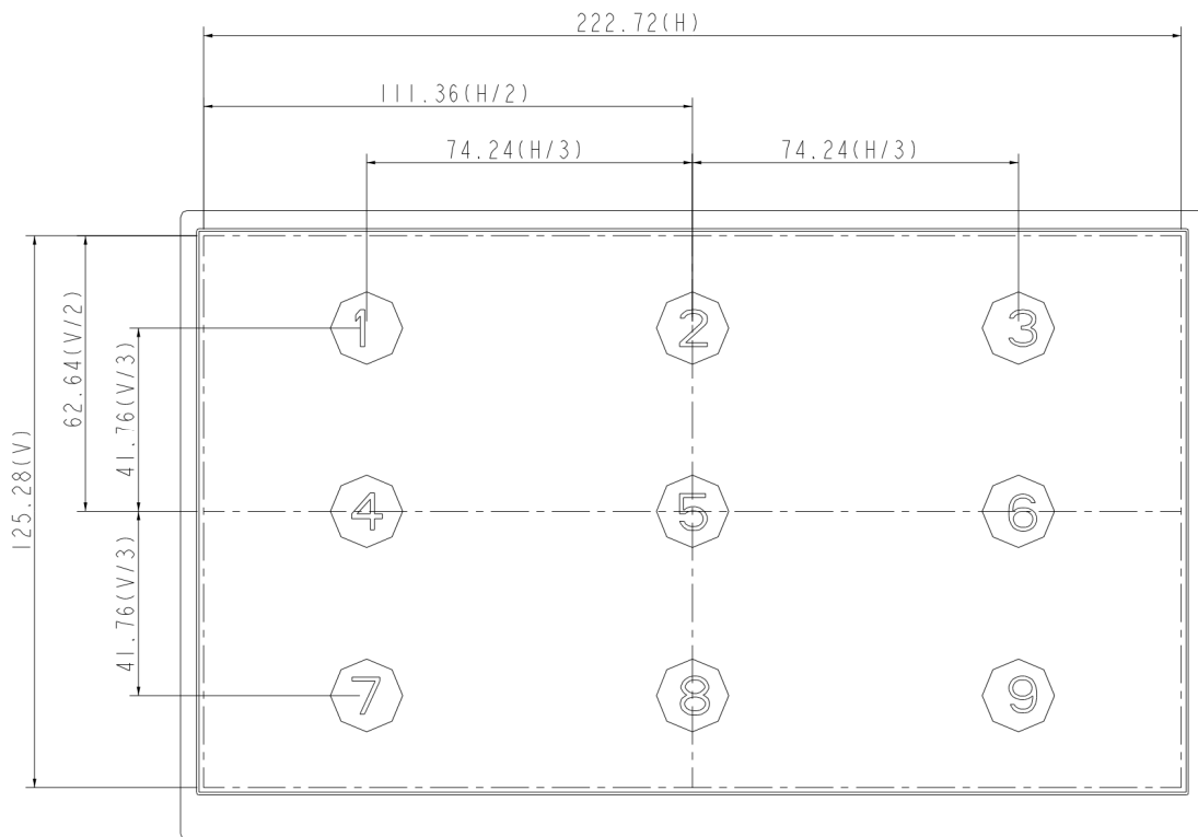
Fig. 9-1 measuring Point
