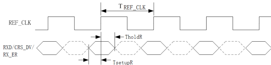
Figure 5-12 RMII Interface Receive Timing
