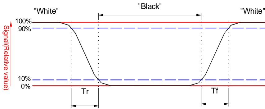
Fig.4-3 Response time
