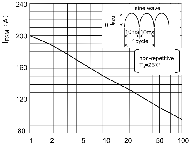
Surge Forward Current Capability
