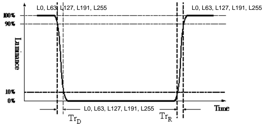
Fig.4-4 Response time
