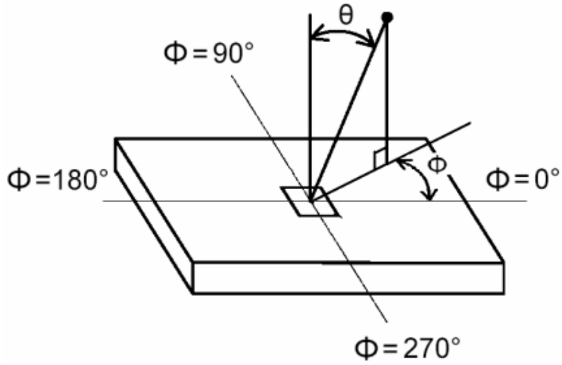
FIG.4-4 Viewing angle
