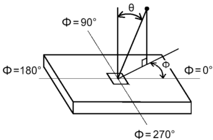
FIG.4 Viewing angle
