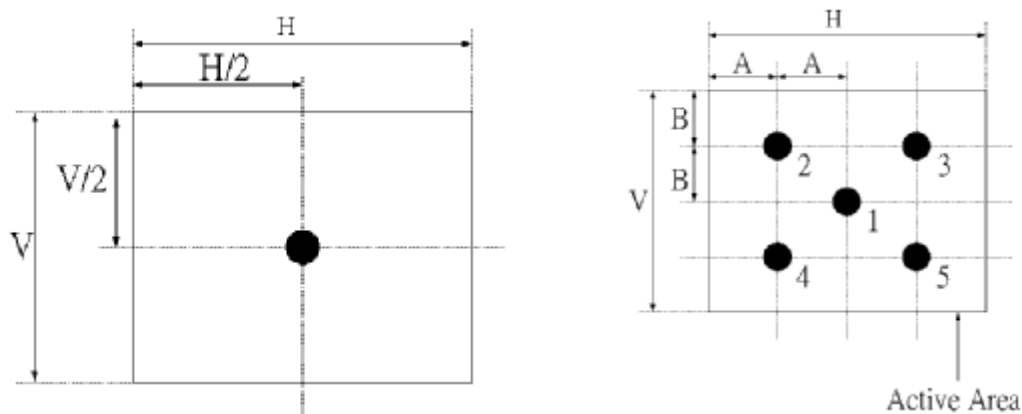
FIG. 2 Luminance
