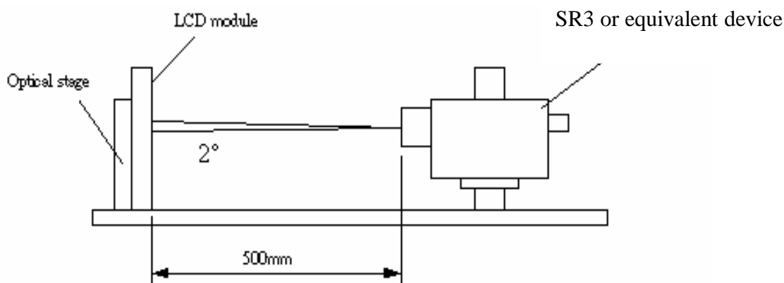
Fig.1 Optical measurement equipment and method.
