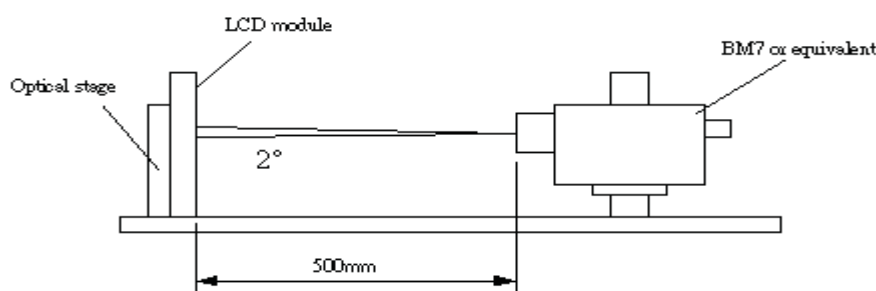
FIG.1 Measurement equipment
