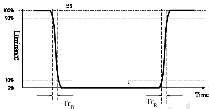
Fig.4-4 Response time
