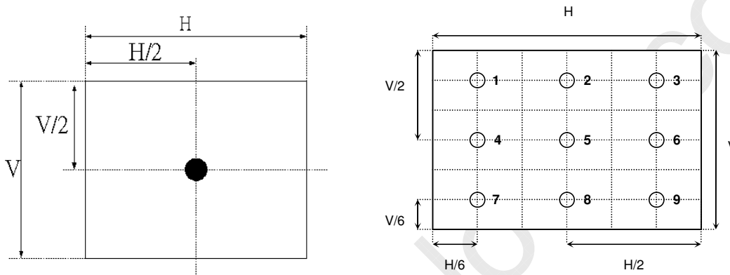
Fig.4-2 Optical measurement point
