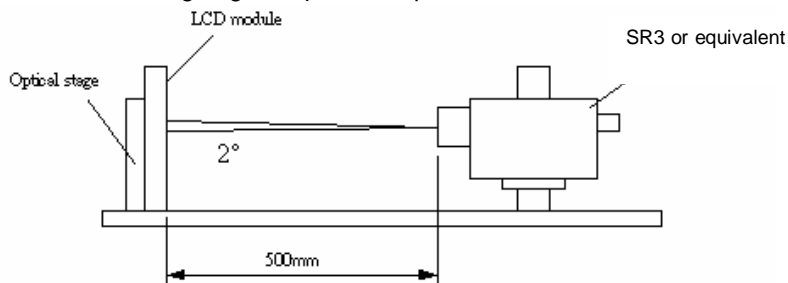
Fig.4-1 Optical measurement method
