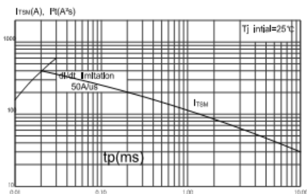
FIG.5: Non-repetitive surge peak on-state current for a sinusoidal pulse with width t_p < 10ms .
