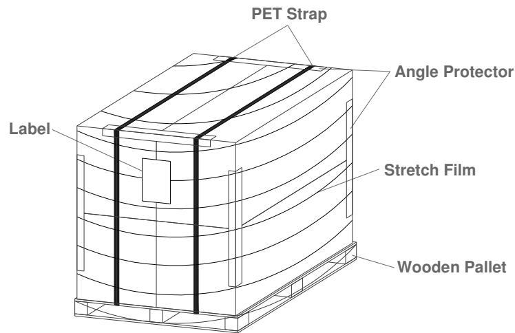
Single pallet packaging illustration
