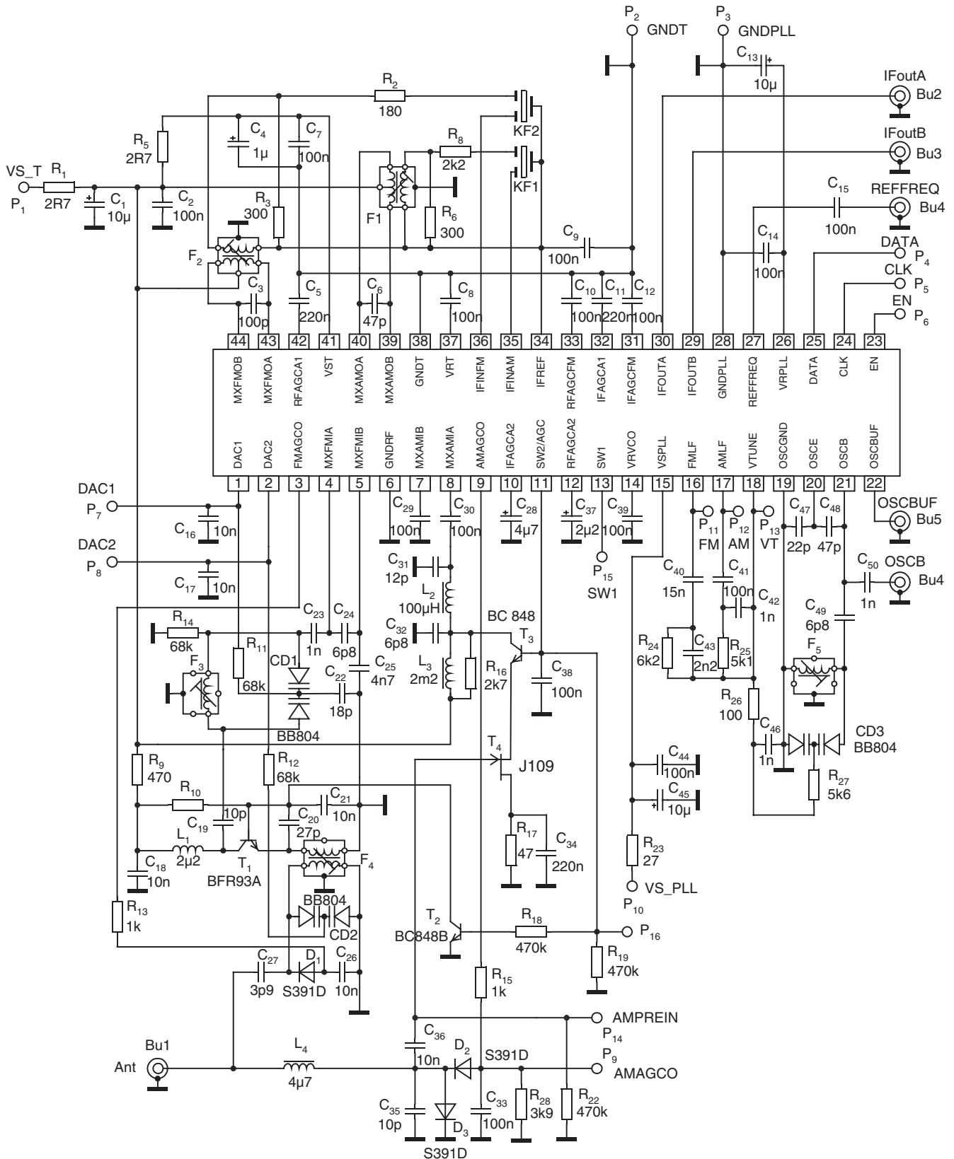
Figure 11-6. Application Circuit
