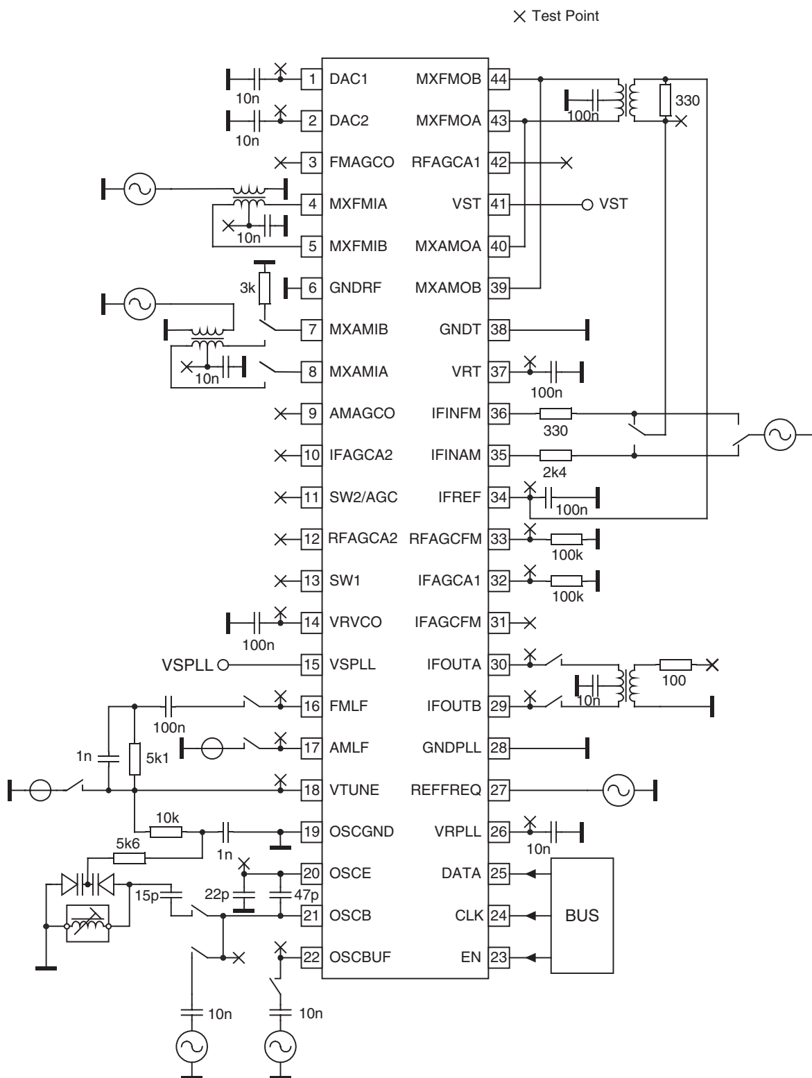
Figure 11-5. Test Circuit
