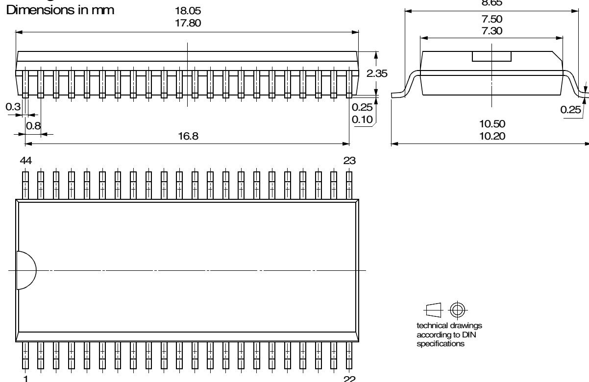
Package SSO44
