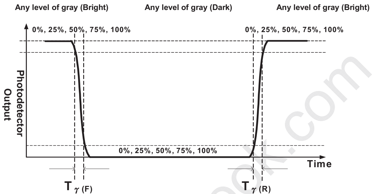
FIG.3 Response Time
