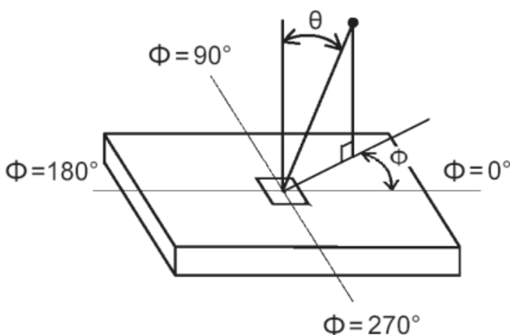
FIG.4 Viewing Angle
