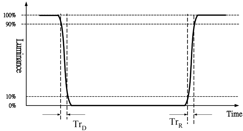
Fig.4-4 Response time
