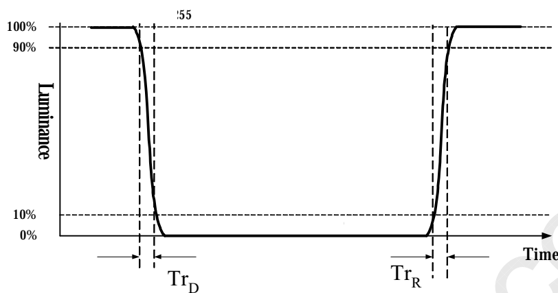
Fig.4-4 Response time
