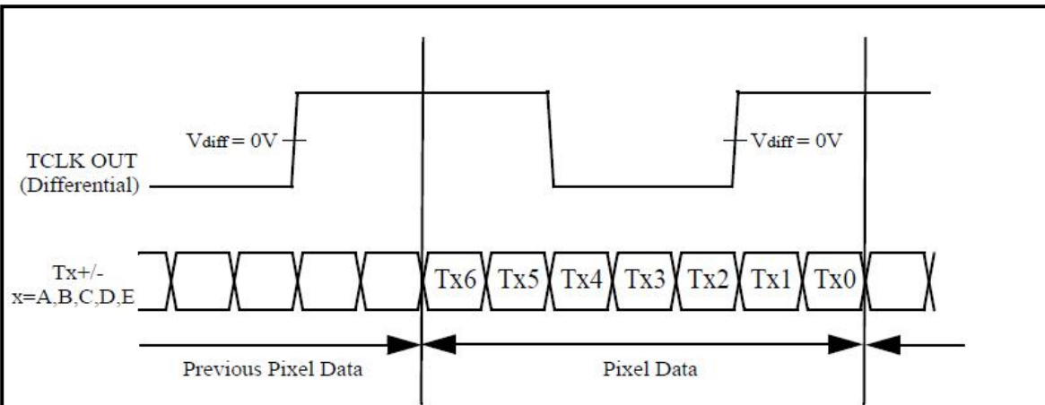
Pixel Data Mapping for VESA Format (6bit, 8bit Application)
