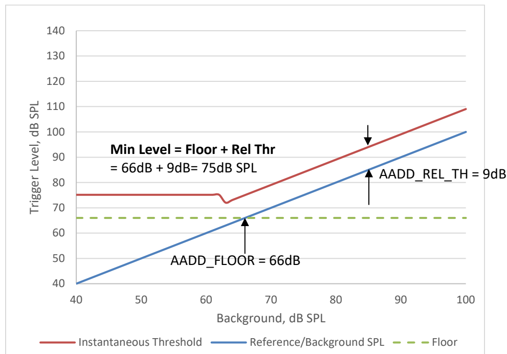
Figure 23. Relative Threshold with floor indicated
