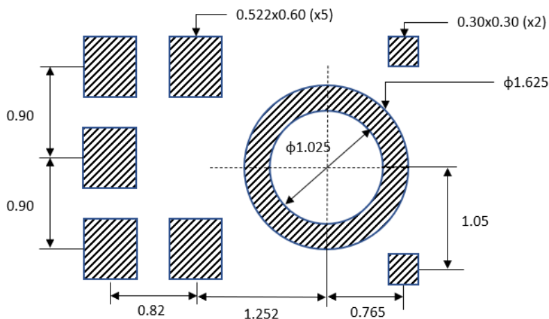
Figure 33. Recommended PCB Land Pattern Layout
