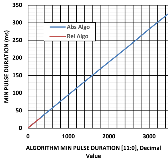
Figure 12. AAD Digital Min Pulse Duration vs Register Value
