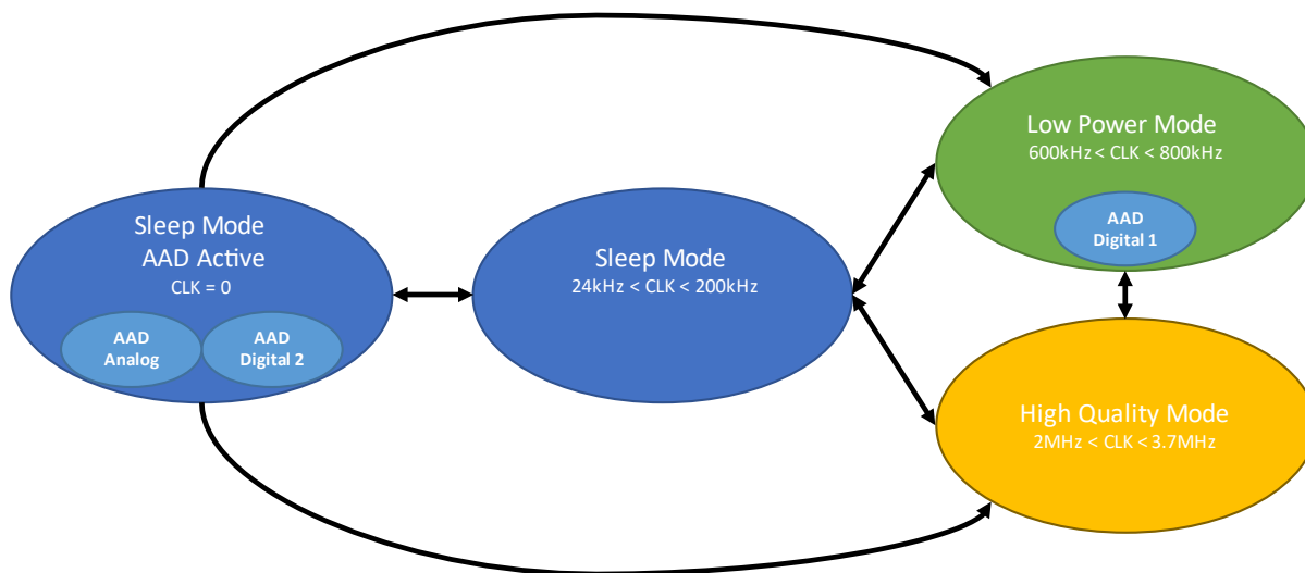
Figure 13. T5848 Mode Transitions
