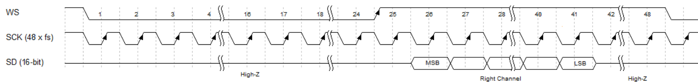
Figure 30. Low Power Mode Stereo Right Channel (LR = 1)
