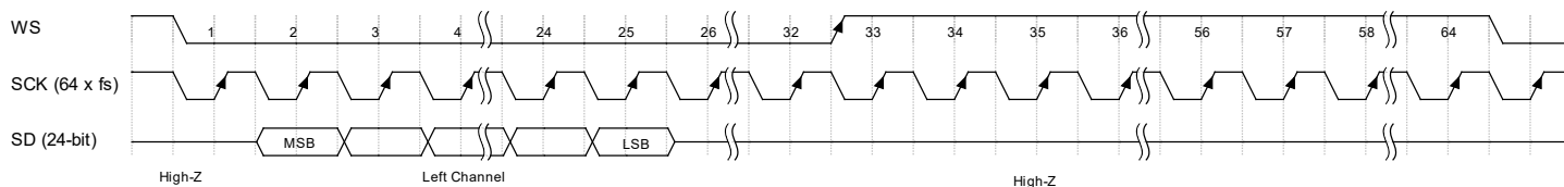
Figure 26. High Quality Mode Stereo Left Channel (LR = 0)
