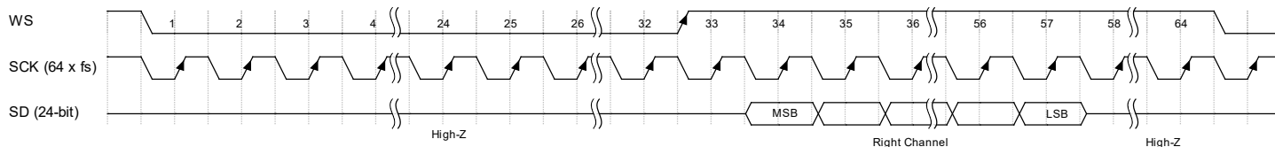
Figure 27. High Quality Mode Stereo Right Channel (LR = 1)
