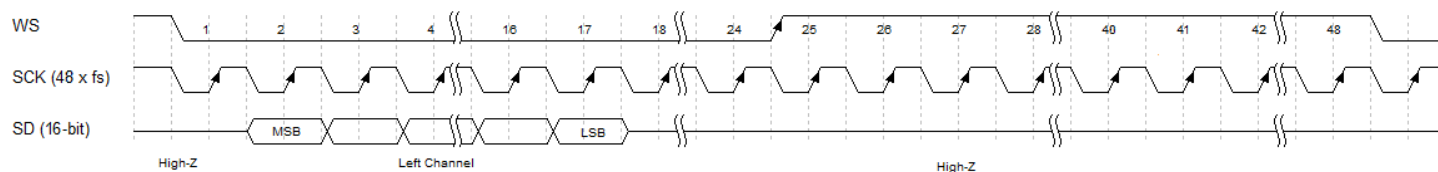
Figure 29. Low Power Mode Stereo Left Channel (LR = 0)
