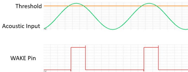
Figure 21. AAD A Threshold level and WAKE pin activation
