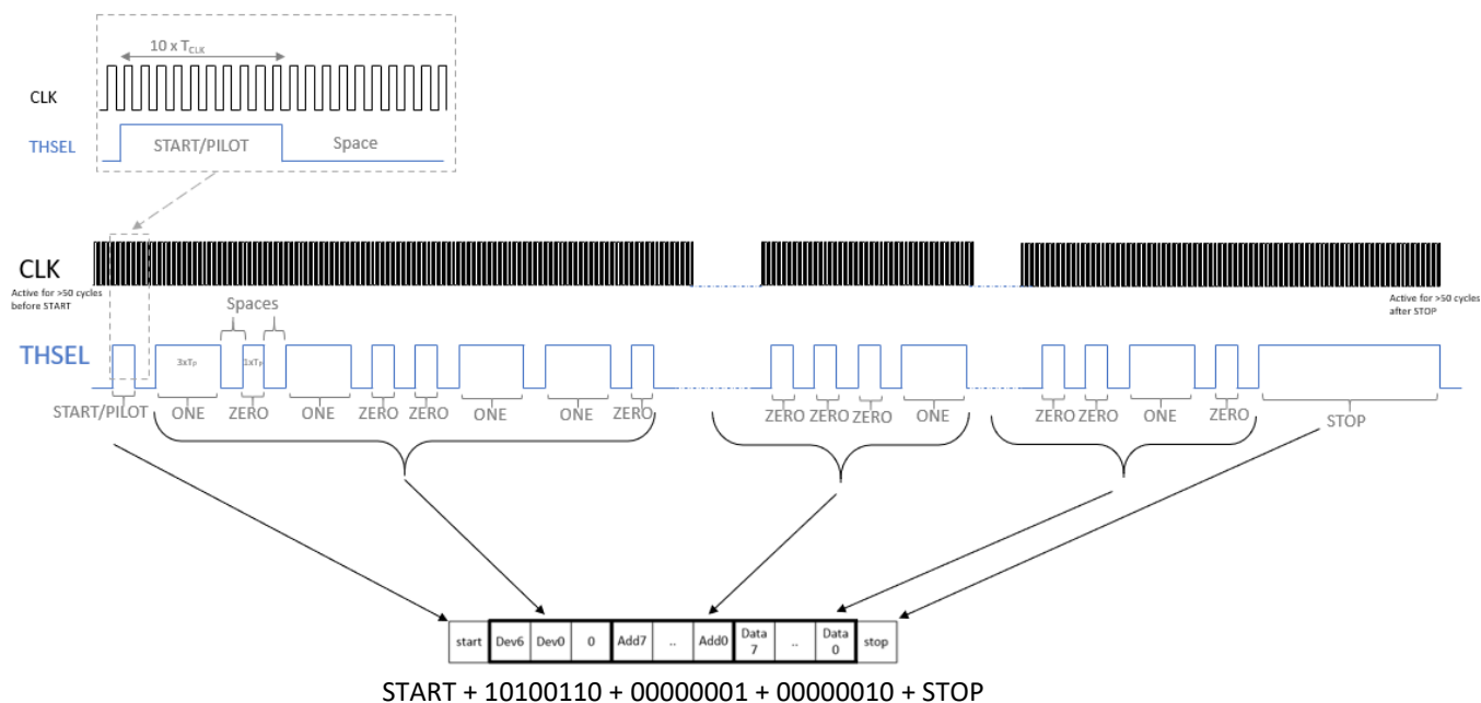
Figure 20. Expanded Timing diagram example showing start, 3 x 8 bit values and stop being written to the device, with the low level translation of each bit to their respective symbols.
