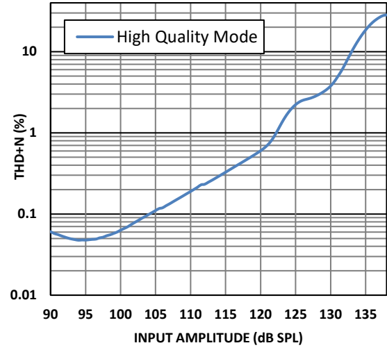
Figure 5. THD + N High Quality Mode – 1 kHz Input
