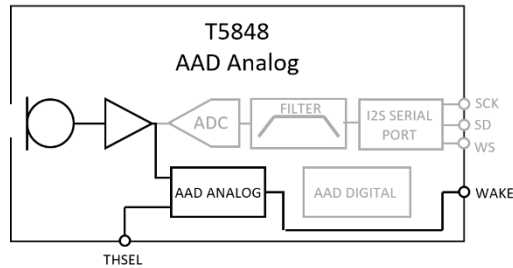
Figure 14. Block Diagram for AAD Analog Operation
