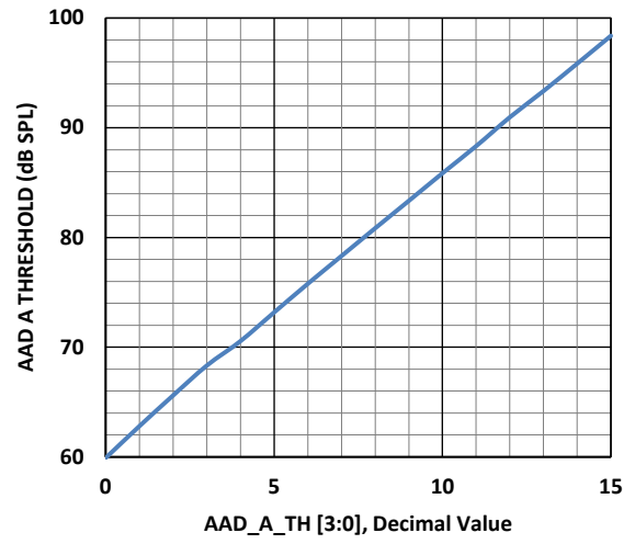
Figure 9. AAD Analog Threshold vs Register Value
