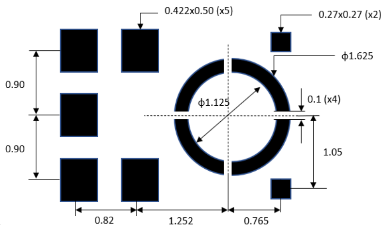
Figure 34. Suggested Solder Paste Stencil Pattern Layout
