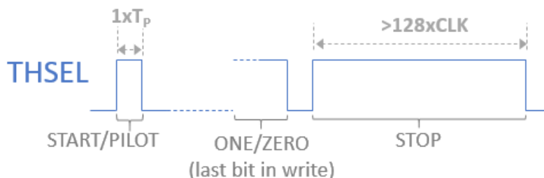
Figure 18. Write termination with Stop
