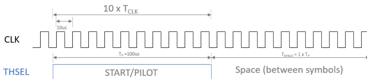
Figure 19. Timing diagram for example above showing relationship between THSEL pilot and CLK
