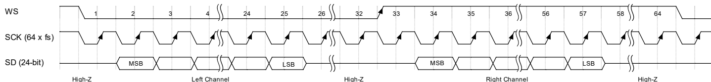
Figure 25. High Quality Mode Stereo Output I 2 S Format
