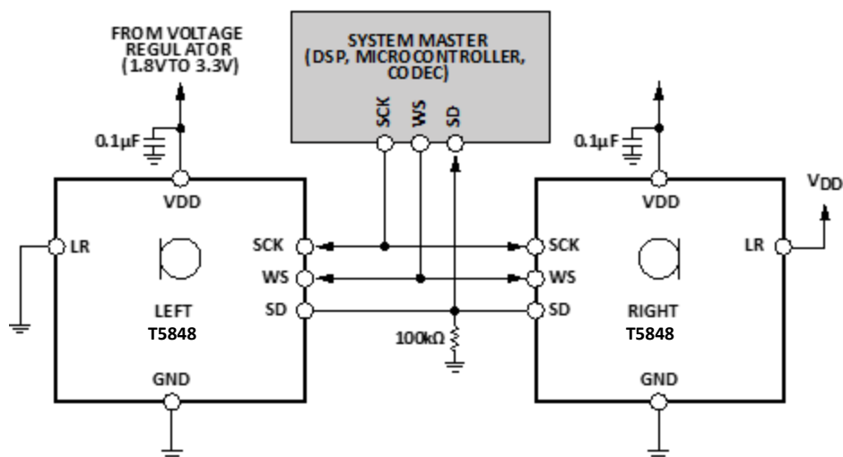
Figure 24. System Block Diagram
