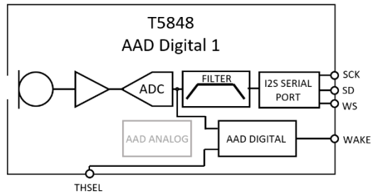
Figure 15. Block Diagram for AAD Digital 1 Operation
