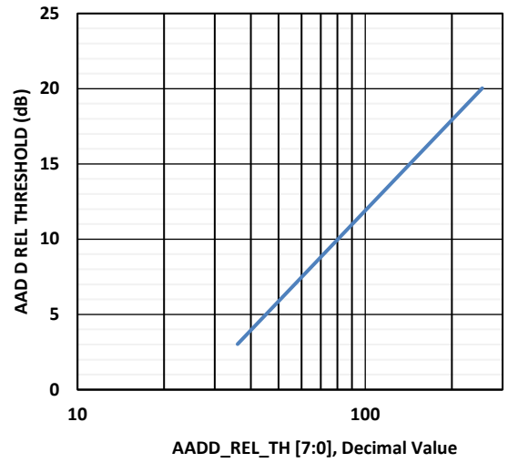
Figure 11. AAD Digital 1,2 Relative Threshold vs Register Value
