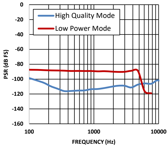
Figure 8. Power Supply Rejection (PSR) vs. Frequency
