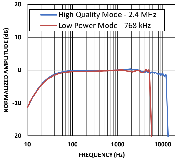
Figure 4. Typical Audio Frequency Response
