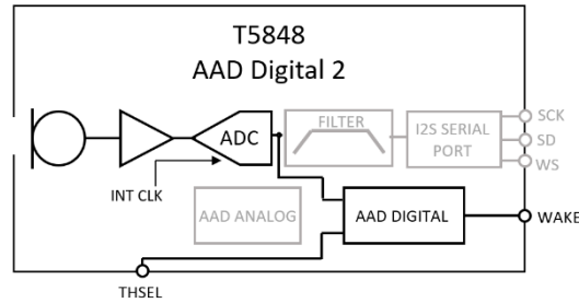
Figure 16. Block Diagram for AAD Digital 2 Operation
