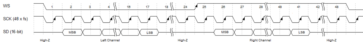
Figure 28. Low Power Mode Stereo Output I 2 S Format
