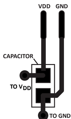
Figure 32. Recommended Power Supply Bypass Capacitor Layout
