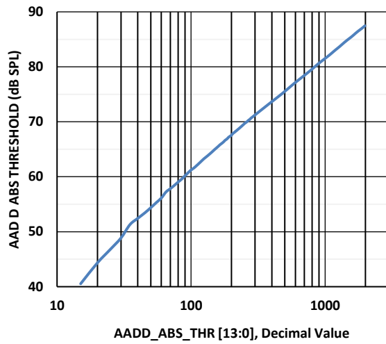
Figure 10. AAD Digital 1,2 Absolute Threshold vs Register Value
