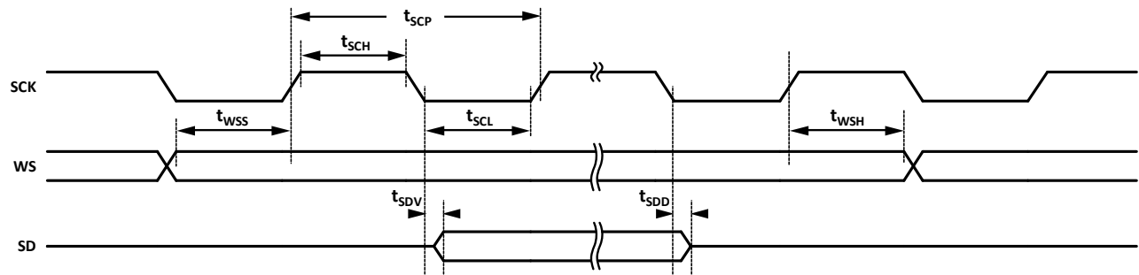
Figure 1. I 2 S Output Timing
