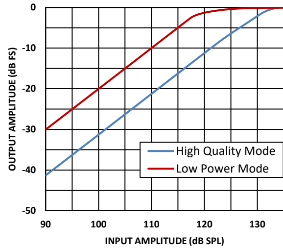
Figure 7. Linearity
