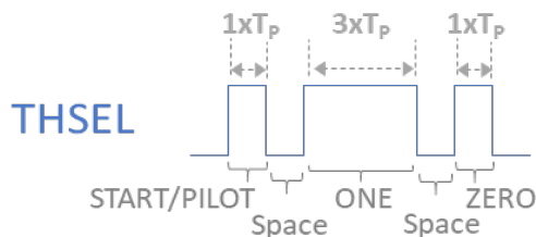
Figure 17. Example write on THSEL followed by a single bit Zero and One relative to the PILOT
