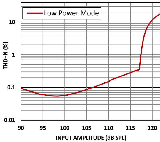
Figure 6. THD + N Low Power Mode – 1 kHz Input
