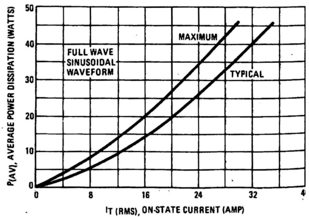
FIGURE 2 – POWER DISSIPATION
