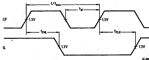
Fig. 2 - Master Reset Pulse Width, Master Reset to Output Delay and Master Reset to Clock Recovery Time
