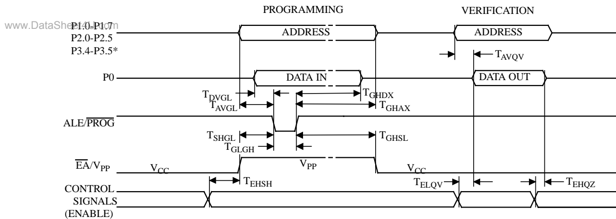
Figure 44. EPROM Programming and Verification Waveforms
