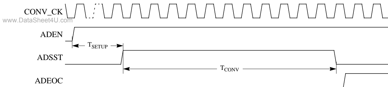
Figure 29. Timing Diagram
