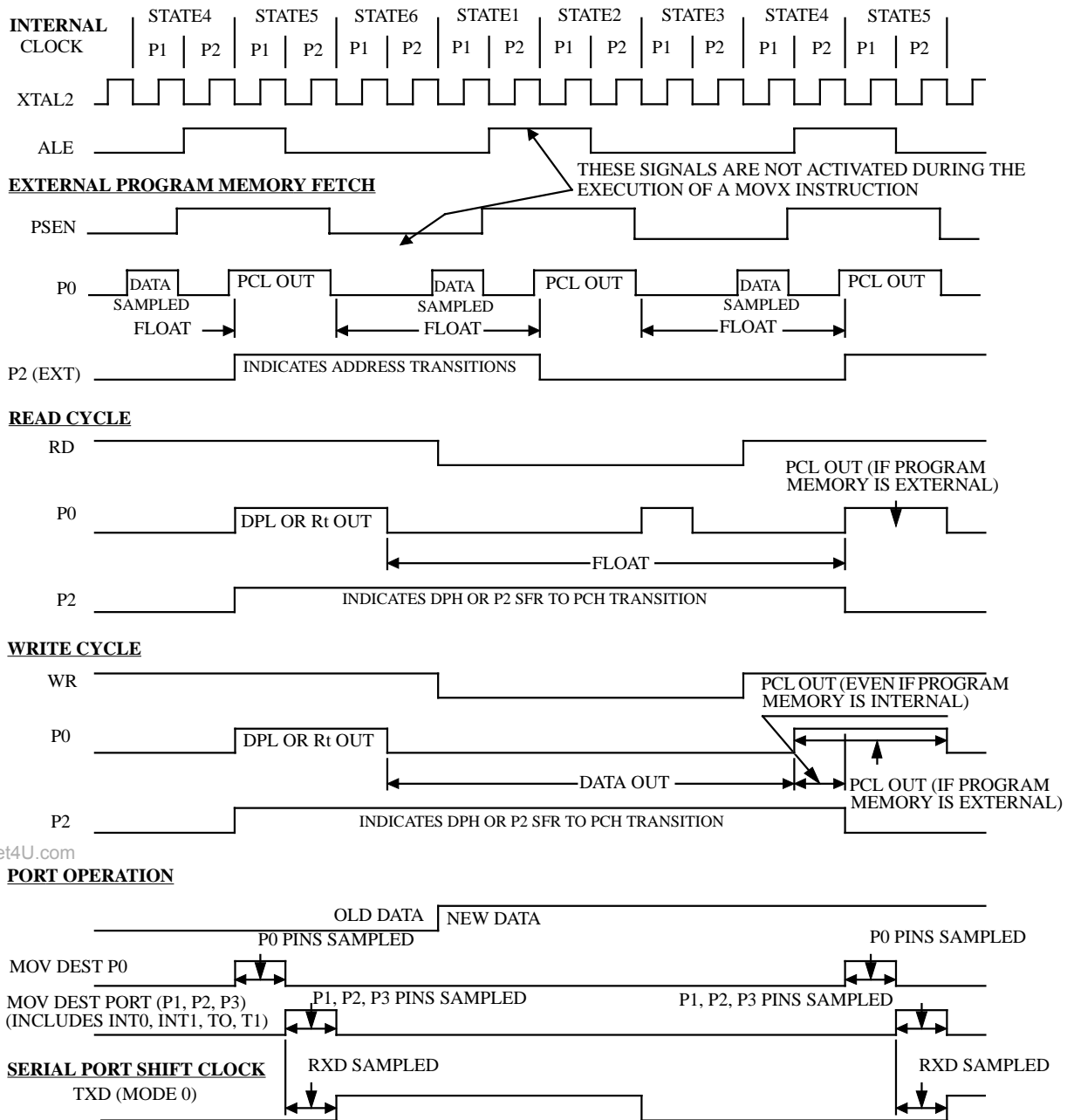
Figure 48. Clock Waveforms
