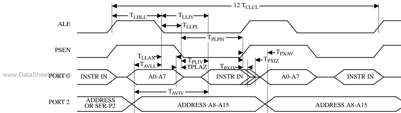
Figure 40. External Program Memory Read Cycle
