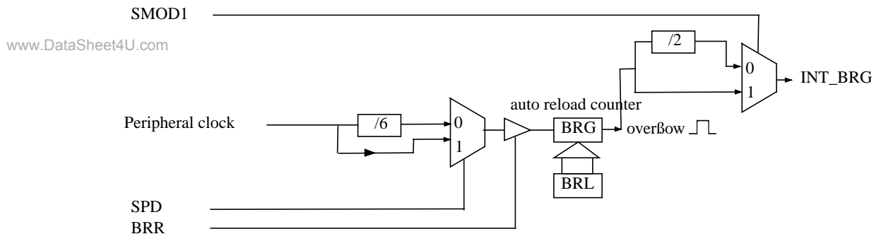
Figure 14. Internal Baud Rate Generator
