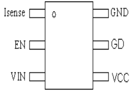
T8305AX SOT23-6
