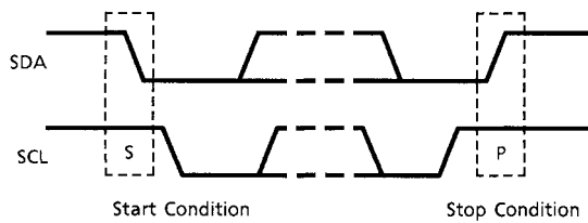
(1) Start and Stop Condition
