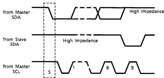
(3) Acknowledge
