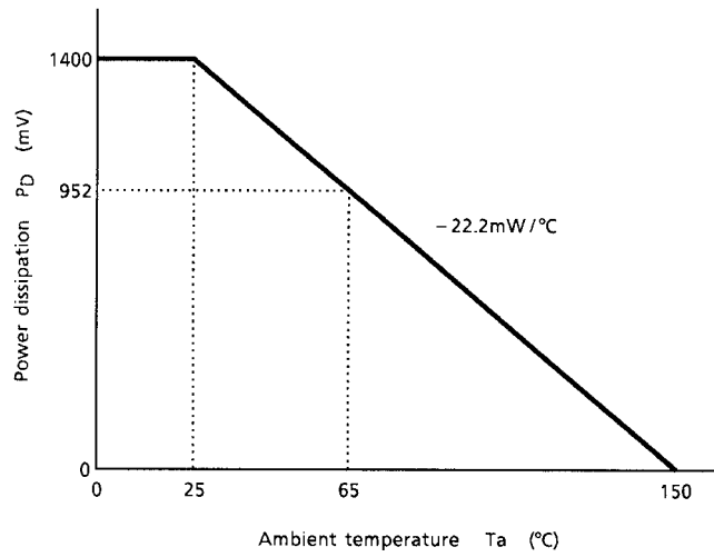
Figure 1 Temperature decrease curve of power dissipation
