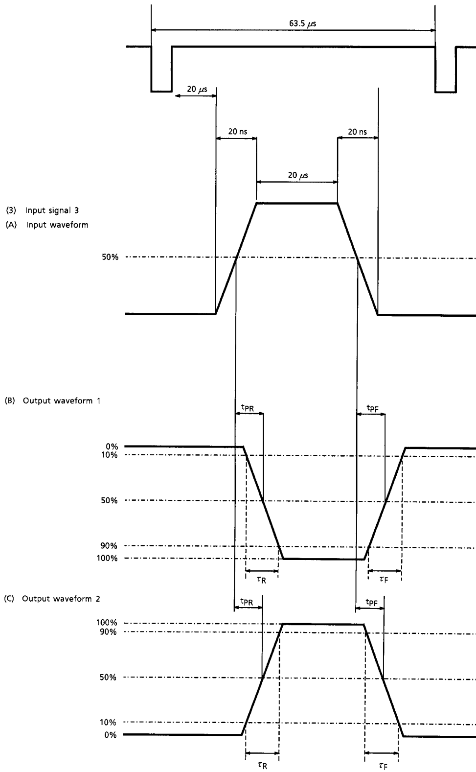
Fig.T-2 Test pulses for TA1310BN text stage
