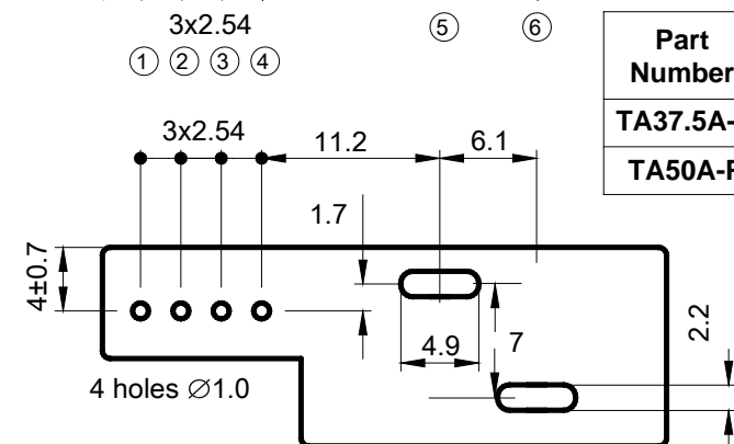
TA37.5A-P..TA50A-P PCB mounting hole layout
