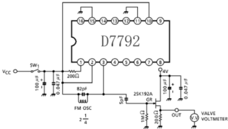
TEST CIRCUIT 2
