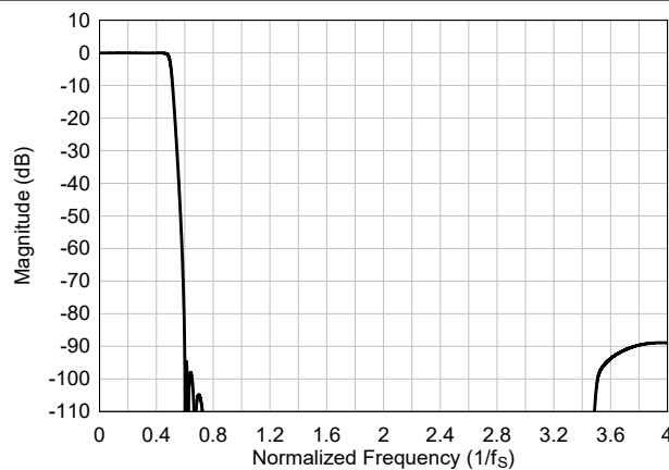
Figure 6-52. Ultra-Low-Latency interpolation Filter Magnitude Response
