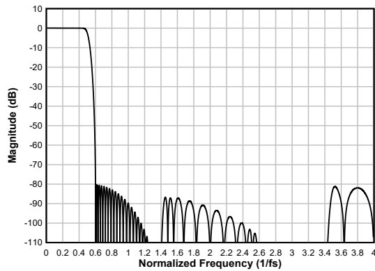
Figure 6-64. Linear-phase Decimation Filter Magnitude Response
