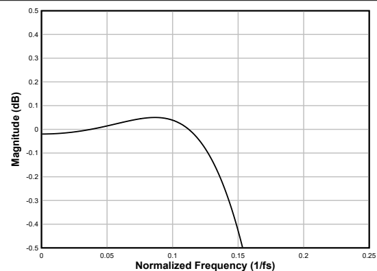
Figure 6-79. Linear-phase Decimation Filter Pass-Band Ripple
