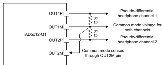
Figure 6-16. Psuedo-differential Output Connection with External Common-Mode Sense (OUT1x_CFG[2:0] = 3'b101)
