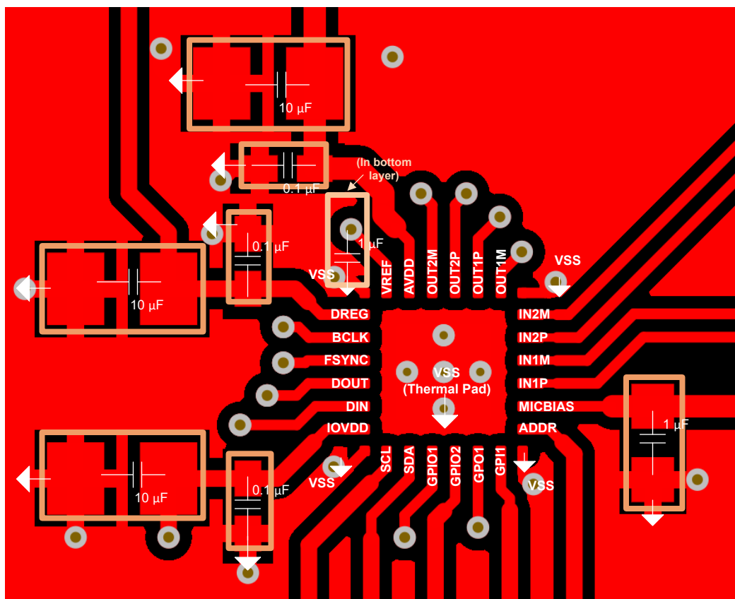
Figure 8-5. Example Layout
