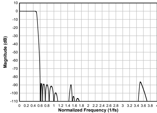
Figure 6-94. Ultra Low-latency Decimation Filter Magnitude Response
