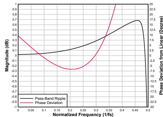
Figure 6-93. Ultra Low-latency Decimation Filter Pass-Band Ripple and Phase Deviation
