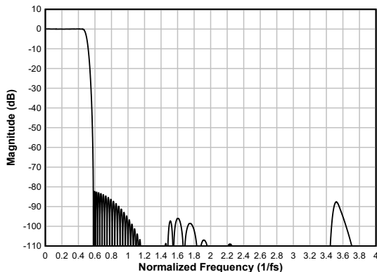
Figure 6-70. Linear-phase Decimation Filter Magnitude Response
