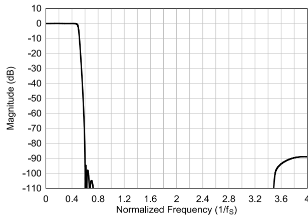
Figure 6-50. Ultra-Low-Latency interpolation Filter Magnitude Response
