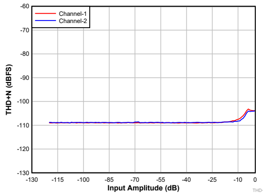
Figure 8-2. DAC THD+N Level vs Input
