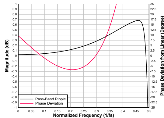
Figure 6-91. Ultra Low-latency Decimation Filter Pass-Band Ripple and Phase Deviation
