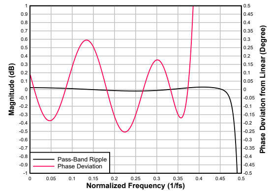
Figure 6-87. Low-latency Decimation Filter Pass-Band Ripple and Phase Deviation
