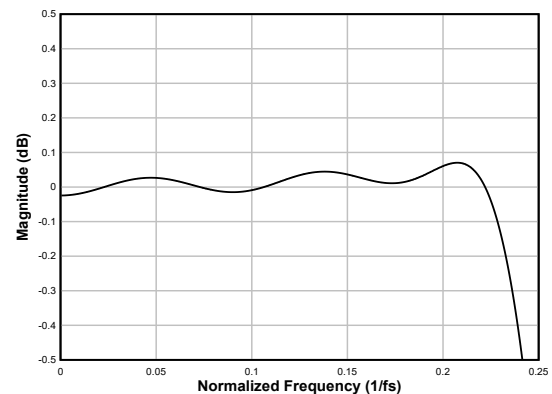
Figure 6-77. Linear-phase Decimation Filter Pass-Band Ripple
