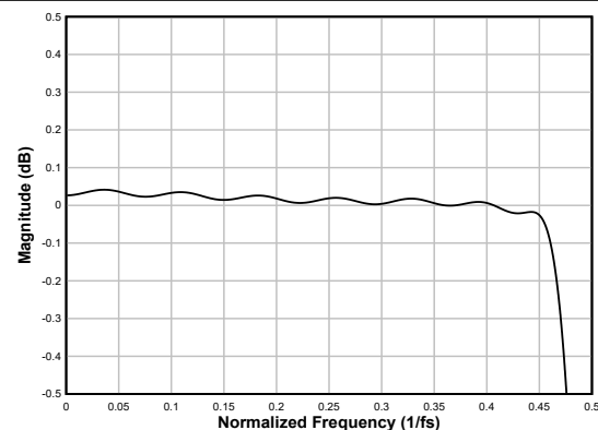
Figure 6-63. Linear-phase Decimation Filter Pass-Band Ripple
