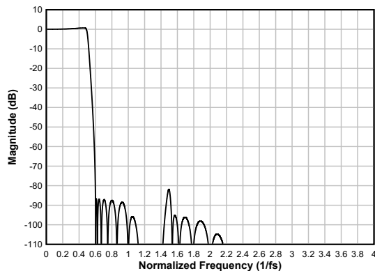
Figure 6-90. Ultra Low-latency Decimation Filter Magnitude Response
