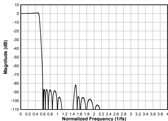
Figure 6-80. Low-latency Decimation Filter Magnitude Response
