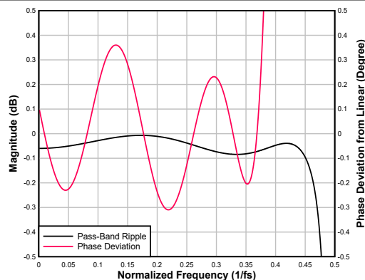
Figure 6-43. Low-latency Interpolation Filter Pass-Band Ripple and Phase Deviation
