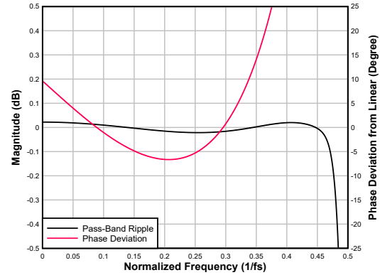
Figure 6-95. Ultra Low-latency Decimation Filter Pass-Band Ripple and Phase Deviation
