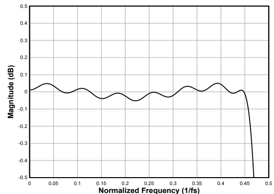
Figure 6-71. Linear-phase Decimation Filter Pass-Band Ripple
