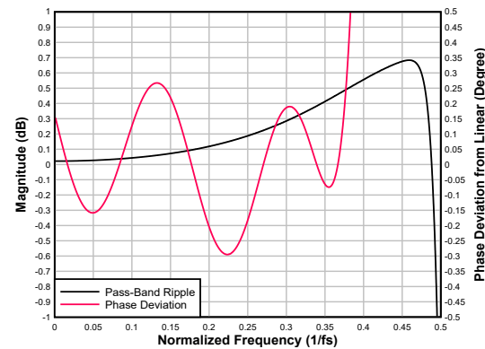
Figure 6-83. Low-latency Decimation Filter Pass-Band Ripple and Phase Deviation
