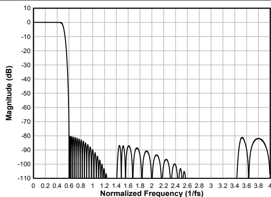
Figure 6-62. Linear-phase Decimation Filter Magnitude Response
