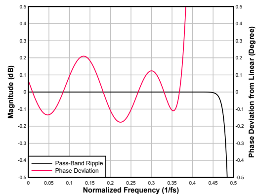
Figure 6-49. Low-latency Interpolation Filter Pass-Band Ripple and Phase Deviation
