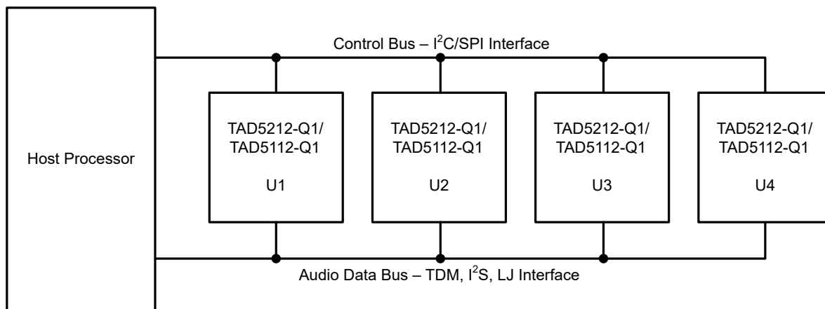
Figure 6-13. Multiple TAD5112-Q1 Devices With Shared Control and Audio Data Buses
