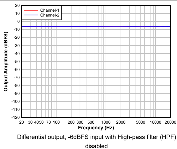
Figure 5-18. DAC Frequency Response
