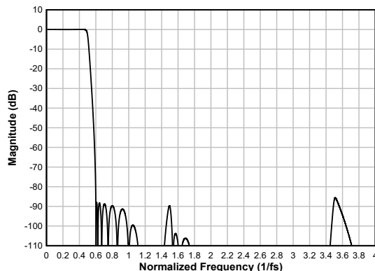
Figure 6-96. Ultra Low-latency Decimation Filter Magnitude Response
