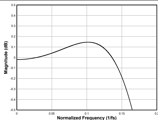
Figure 6-39. Linear-phase Interpolation Filter Pass-Band Ripple
