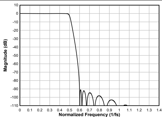
Figure 6-98. Ultra Low-latency Decimation Filter Magnitude Response
