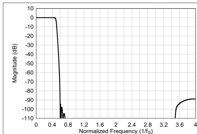
Figure 6-54. Ultra-Low-Latency interpolation Filter Magnitude Response
