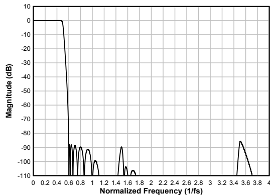
Figure 6-86. Low-latency Decimation Filter Magnitude Response
