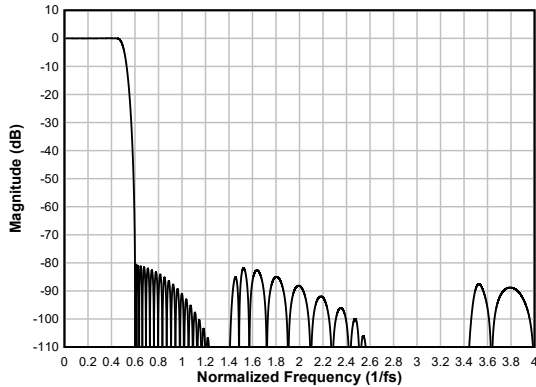
Figure 6-68. Linear-phase Decimation Filter Magnitude Response
