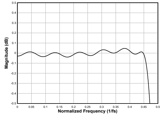
Figure 6-69. Linear-phase Decimation Filter Pass-Band Ripple
