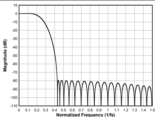
Figure 6-38. Linear-phase Interpolation Filter Magnitude Response
