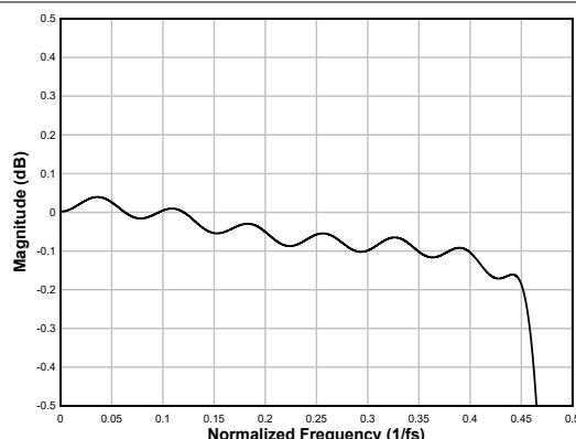
Figure 6-33. Linear-phase Interpolation Filter Pass-Band Ripple
