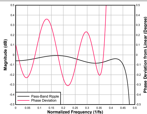
Figure 6-45. Low-latency Interpolation Filter Pass-Band Ripple and Phase Deviation
