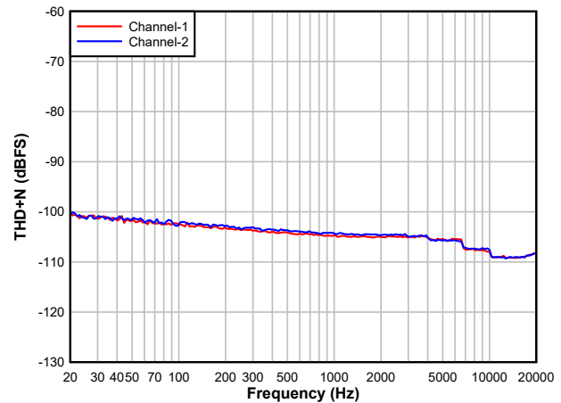
Figure 5-10. DAC THD+N Level vs Frequency
