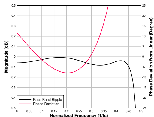
Figure 6-55. Ultra-Low-Latency interpolation Filter Pass-Band Ripple and Phase Deviation
