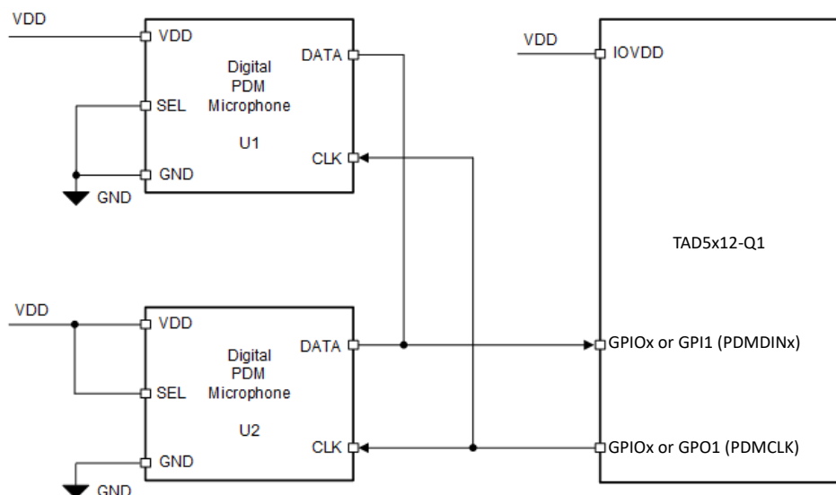
Figure 6-18. Digital PDM Microphones Connection Diagram for the TAD5112-Q1
