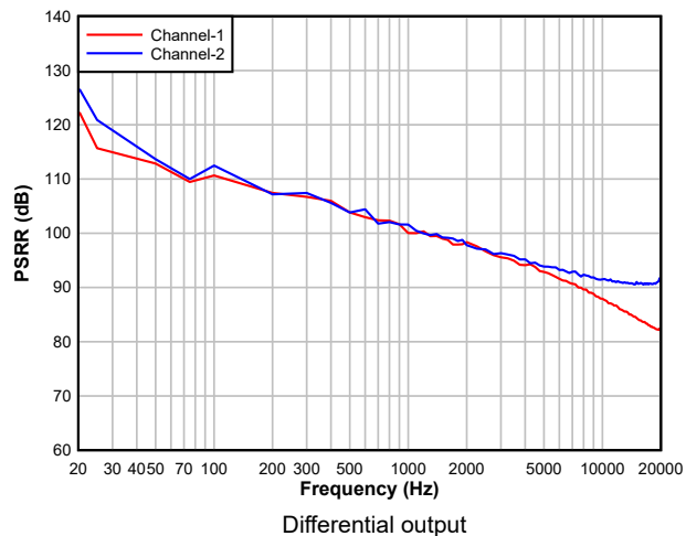
Figure 5-16. DAC PSRR vs Frequency
