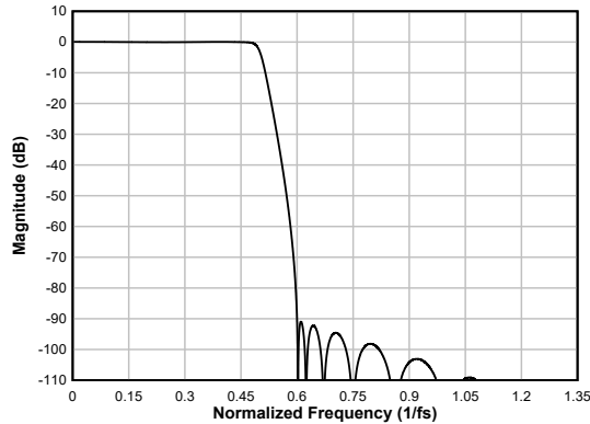
Figure 6-88. Low-latency Decimation Filter Magnitude Response
