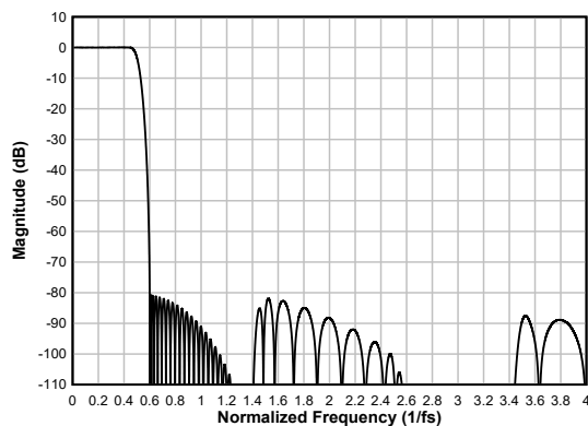
Figure 6-66. Linear-phase Decimation Filter Magnitude Response
