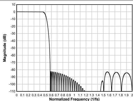
Figure 6-32. Linear-phase Interpolation Filter Magnitude Response
