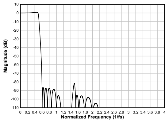
Figure 6-82. Low-latency Decimation Filter Magnitude Response
