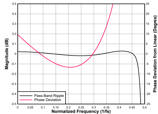
Figure 6-97. Ultra Low-latency Decimation Filter Pass-Band Ripple and Phase Deviation
