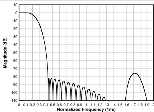
Figure 6-78. Linear-phase Decimation Filter Magnitude Response
