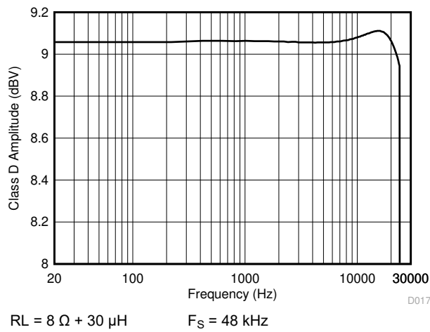
Figure 6-23. Amplitude vs Frequency
