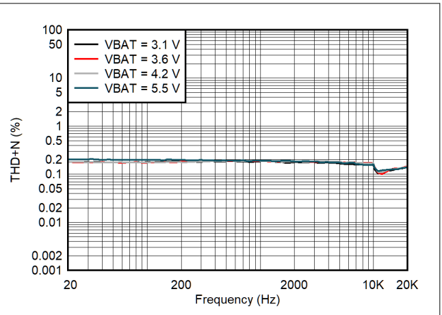
Figure 6-46. I-sense THD+N vs Frequency (QFN Package)
