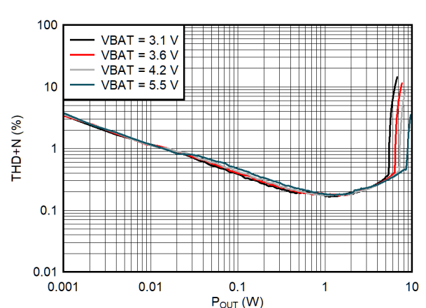
Figure 6-38. I-sense THD+N vs Output Power (QFN Package)
