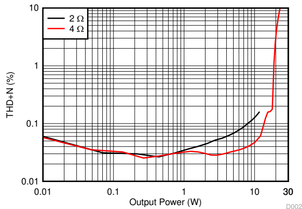
Figure 6-2. THD+N vs Output Power
