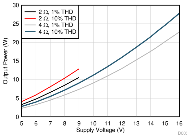
Figure 6-3. Output Power vs PVDD
