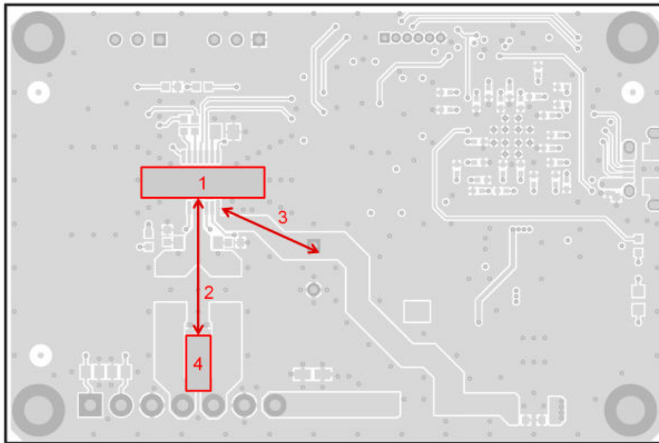
Figure 10-1. Top layer
