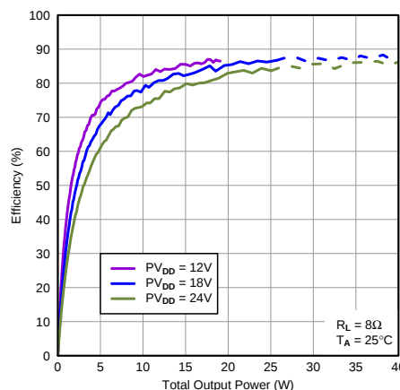
Figure 44. Efficiency vs Total Output Power
