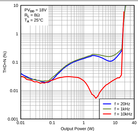
Figure 9. Total Harmonic Distortion + Noise vs Output Power
