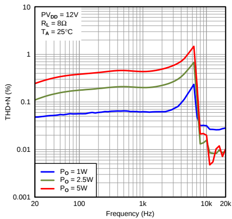
Figure 5. Total Harmonic Distortion + Noise vs Frequency
