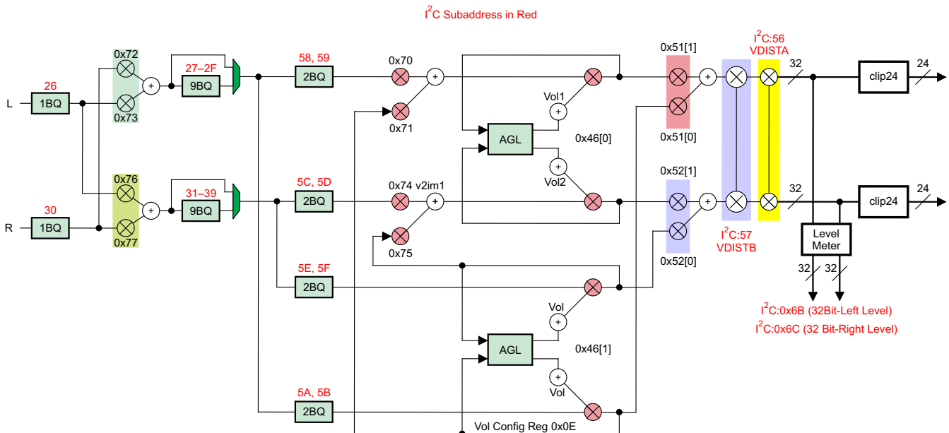
Figure 17. DAP Process Structure
