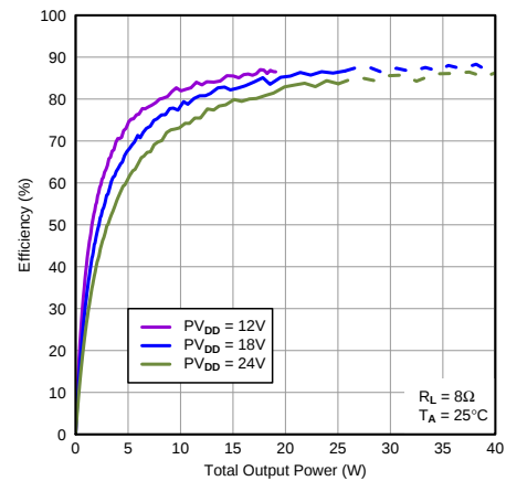
Figure 14. Efficiency vs Total Output Power
