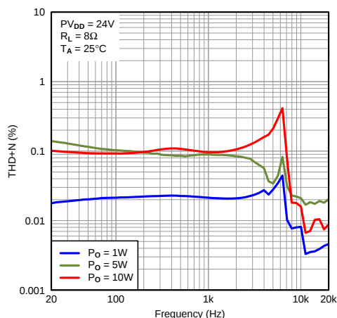
Figure 43. Total Harmonic Distortion + Noise vs Frequency
