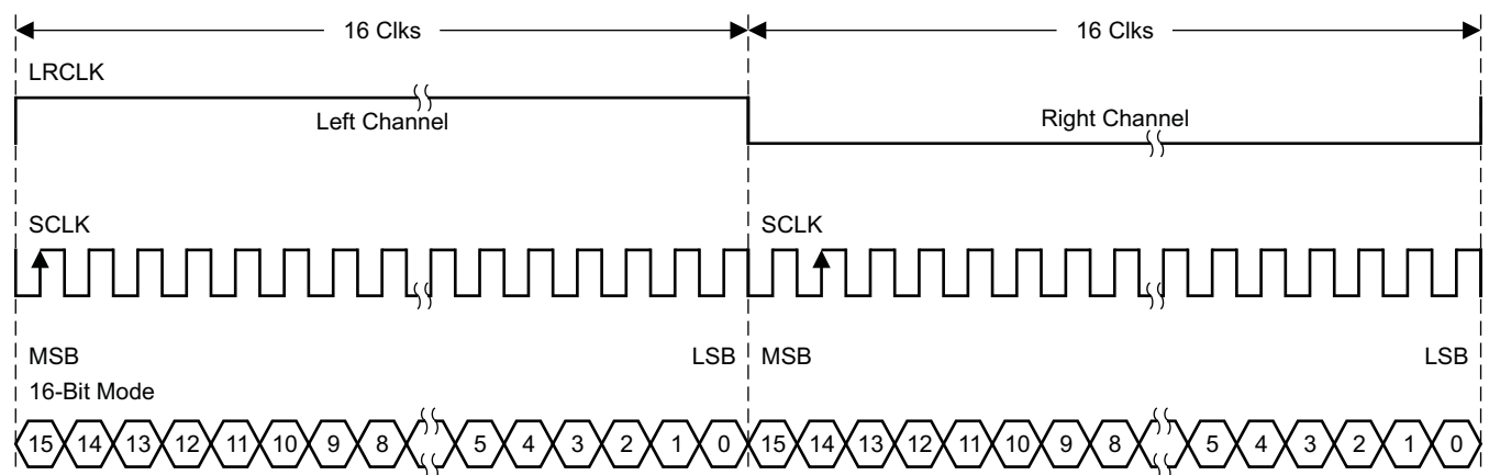
Figure 28. Left-Justified 32-f s Format
