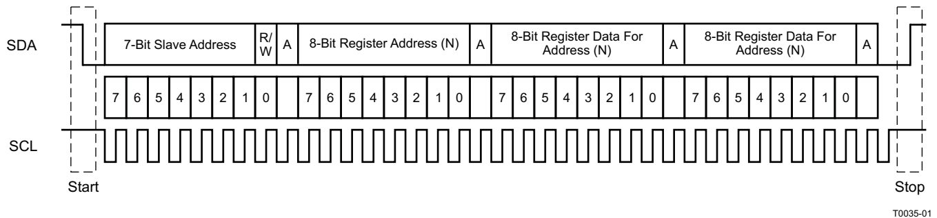
Figure 18. Typical I 2 C Sequence
