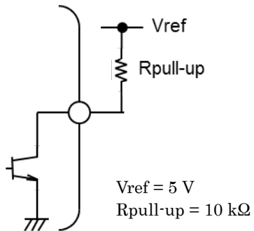
Test circuit (5)
