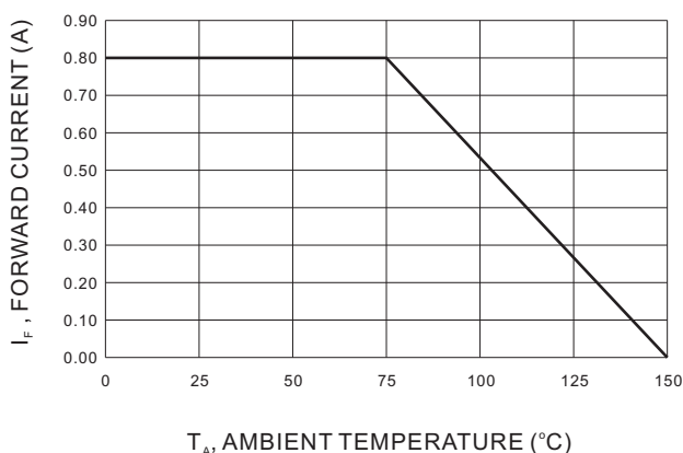
FIG 3- DERATING CURVE
