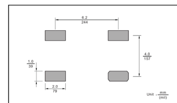
The recommended mounting pad size
